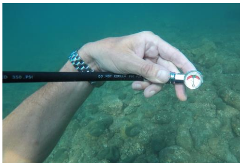
The system includes a remote pressure gauge to monitor the cylinder pressure
